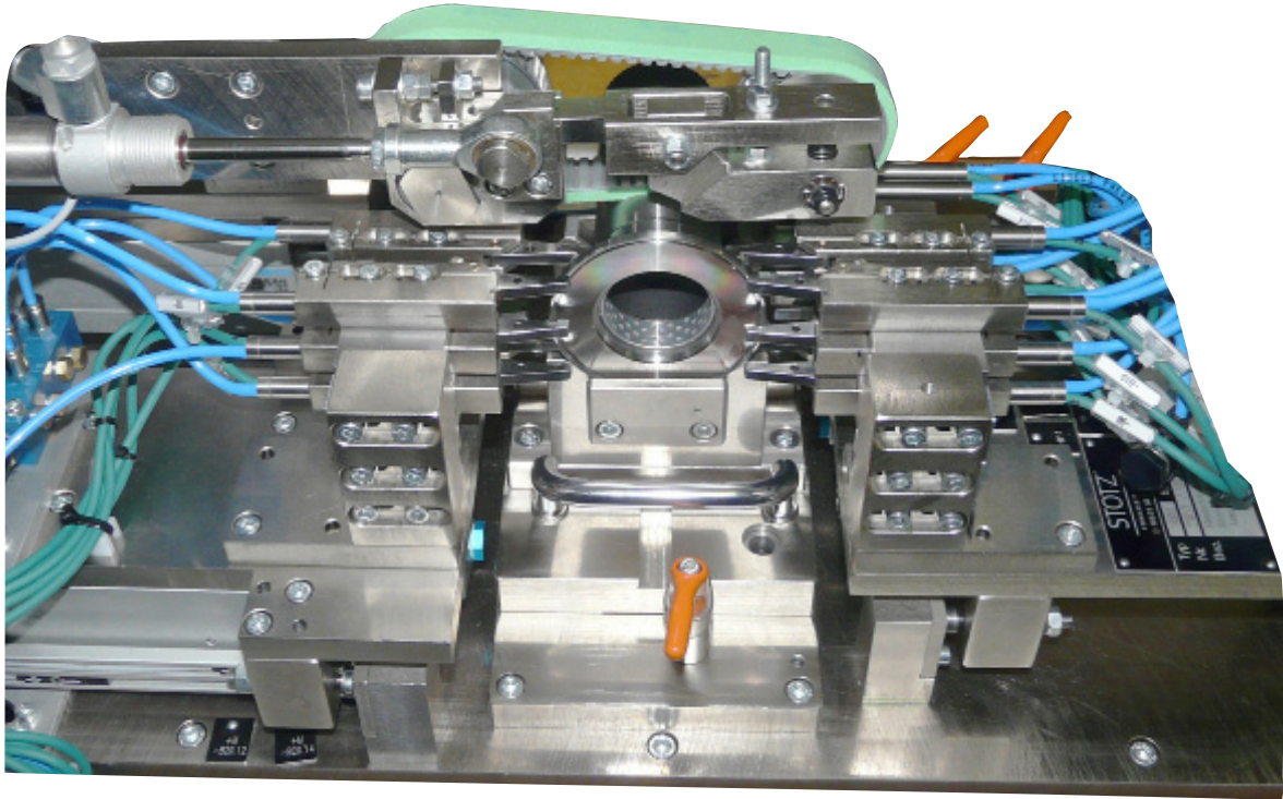
Examination of I.D. diameter
