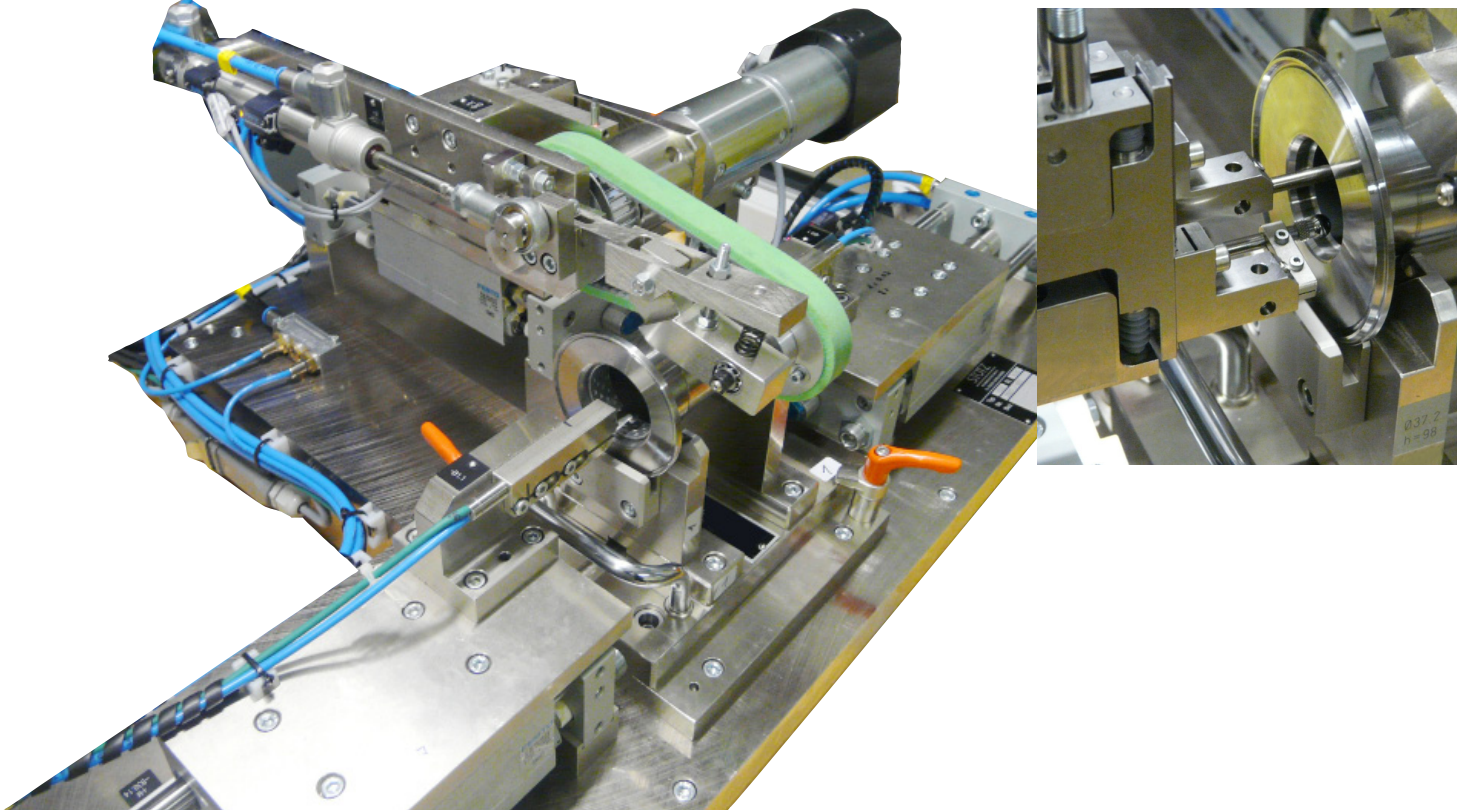
Examination of I.D. diameter
